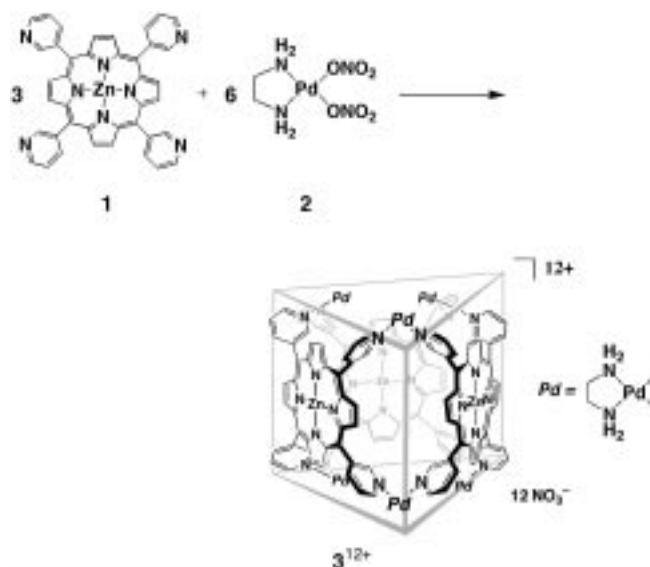
Scheme 1. Self-assembly of porphyrin prism 3^{12+} .
